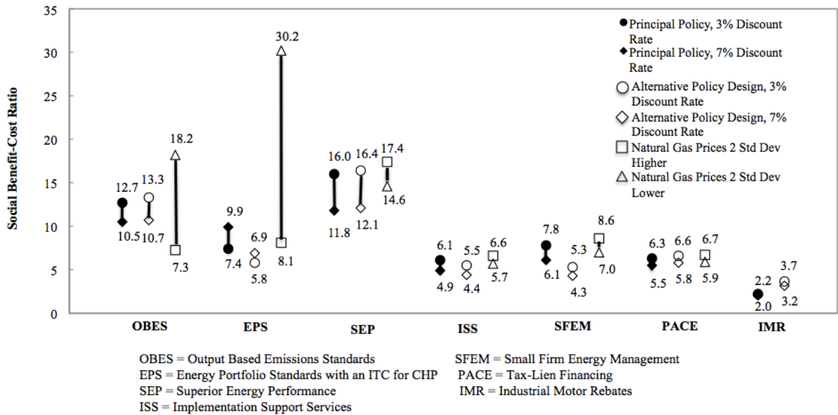
Figure 9. Sensitivity Analysis of Key Risk Factors Using Social Benefit-Cost Ratios
