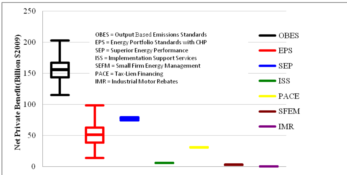
Figure 7. Box and Whisker Plot of Net Private Benefit (7% discount rate)
